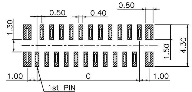
RECOMMENDED P.C.BOARD LAYOUT A TYPE
