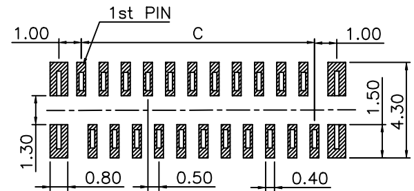
RECOMMENDED P.C.BOARD LAYOUT B TYPE
