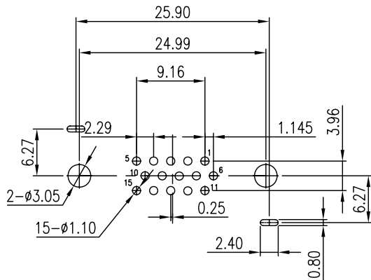
RECOMMENDED P.C.BOARD TOP VIEW
