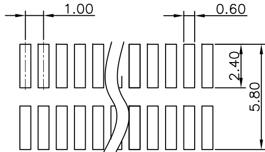
RECOMMENDED PCB LAYOUT TOLERANCE: ±0.05mm
