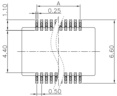
RECOMMENDED P.C.BOARD
