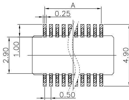
RECOMMENDED P.C.BOARD
