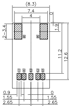
RECOMMENDED P.C. BOARD HOLE LAYOUT
